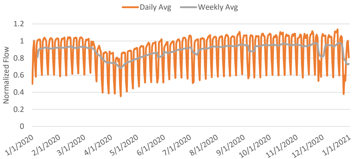
Figure 4-13: SCAB portion of Los Angeles county traffic flow from Caltrans' PeMS. The data is normalized to 2018 traffic flow.
