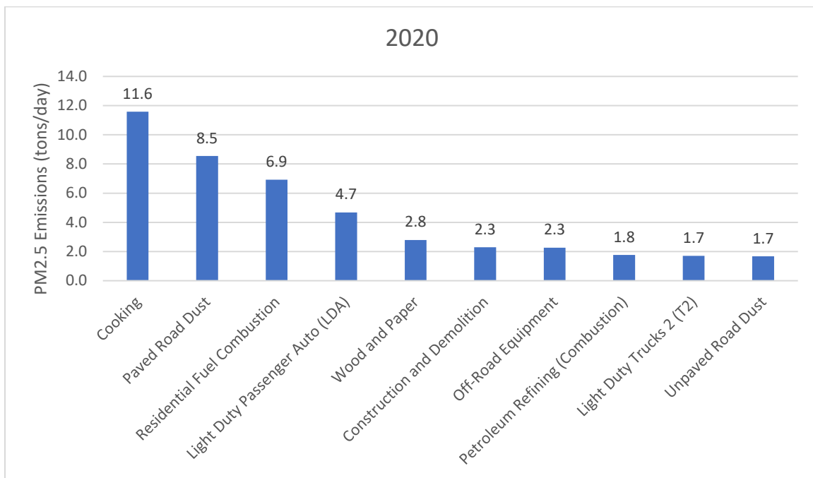
Figure 3-3: Top 10 PM 2.5 sources in 2020
