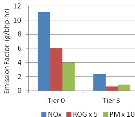
Carl Moyer Program Emission Factors
