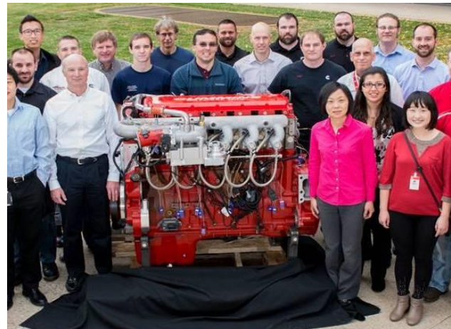
Figure 35: ISX15-G Ultra Low NOx Prototype Engine
