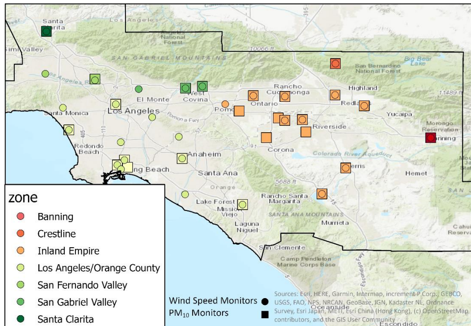
Figure 2-2: Zones sharing similar meteorological characteristics used to identify suspected exceptional events caused by high winds
