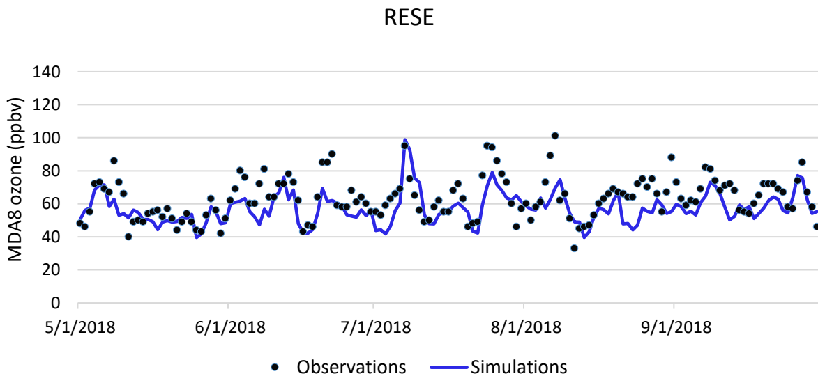
FIGURE III-A-20 2018 MDA8 OZONE MODEL PREDICTION AND MEASUREMENT COMPARISON AT RESEDA
