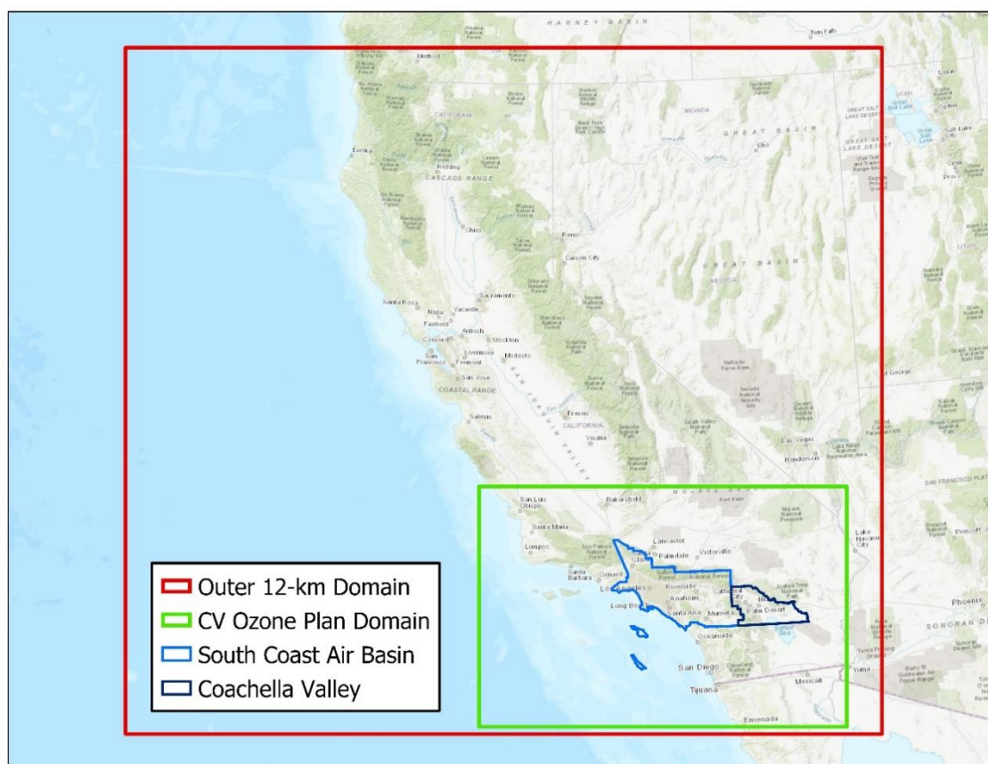
FIGURE 5-1 MODELING DOMAINS FOR THE MODELING OF OZONE IN THE COACHELLA VALLEY
