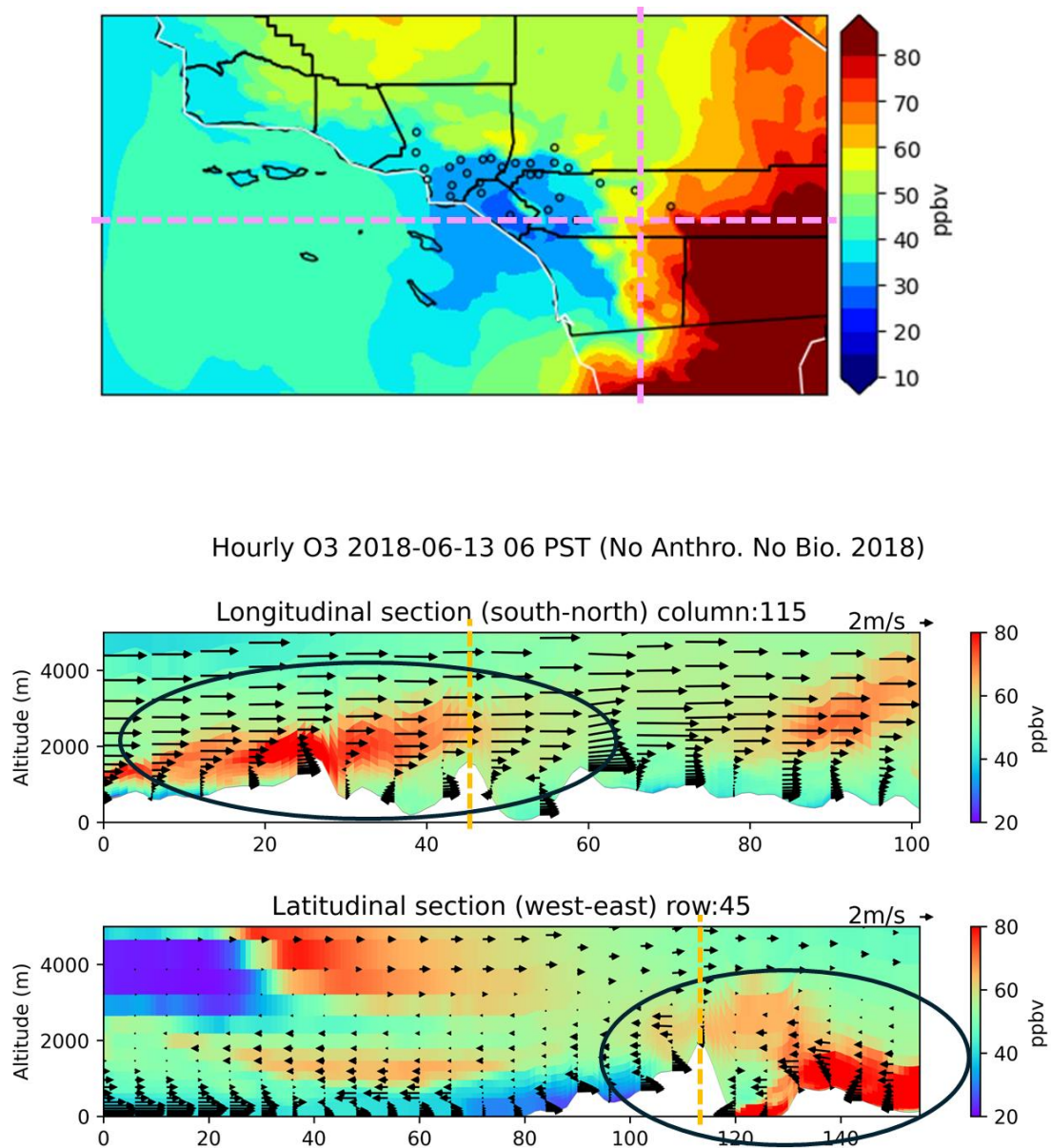
FIGURE 5-8 EXAMPLE OF OZONE TRANSPORT EVENT FROM THE SOUTHERN BOUNDARY (TOP) AND CROSS SECTION OF OZONE CONCENTRATION ALONG THE CROSS-SECTIONS HIGHLIGHTED (BOTTOM)
