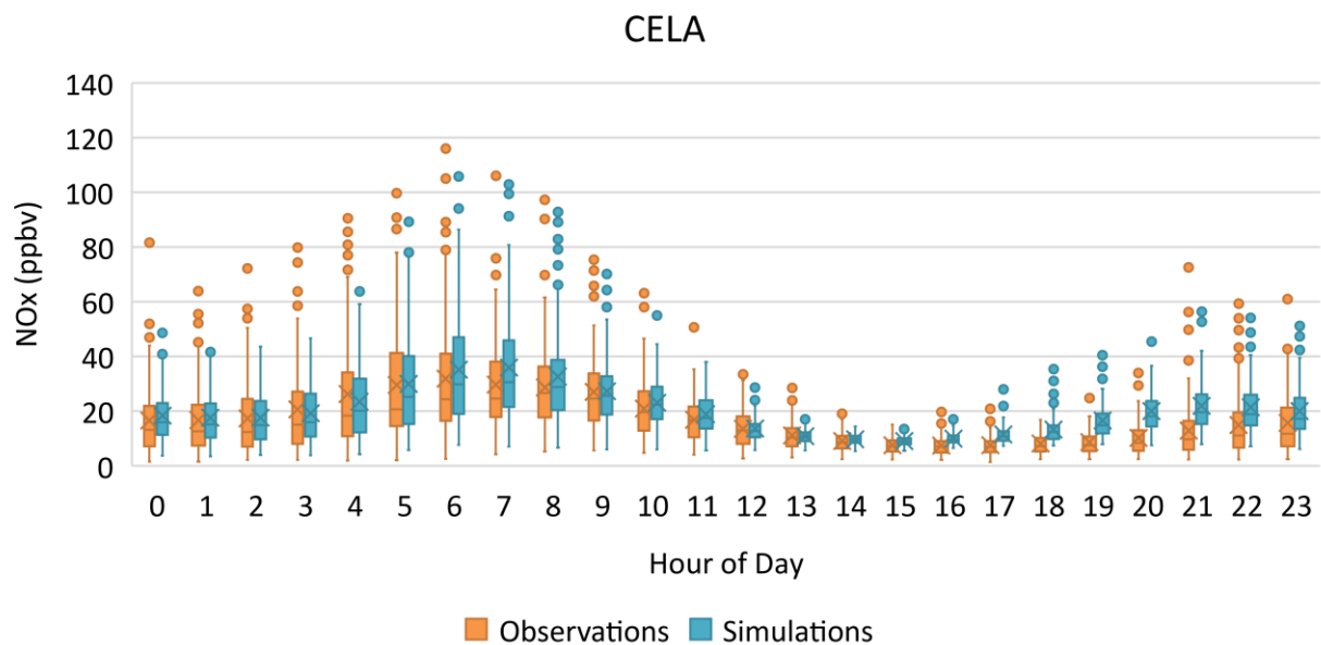
FIGURE III-E-4 BOX PLOTS OF OBSERVED VS. PREDICTED HOURLY NO x DURING MAY 1 ST TO SEPTEMBER 30 TH , 2018, AT CENTRAL LOS ANGELES. HORIZONTAL LINES INDICATE 25 TH , 50 TH (MEDIAN), AND 75 TH PERCENTILES.
