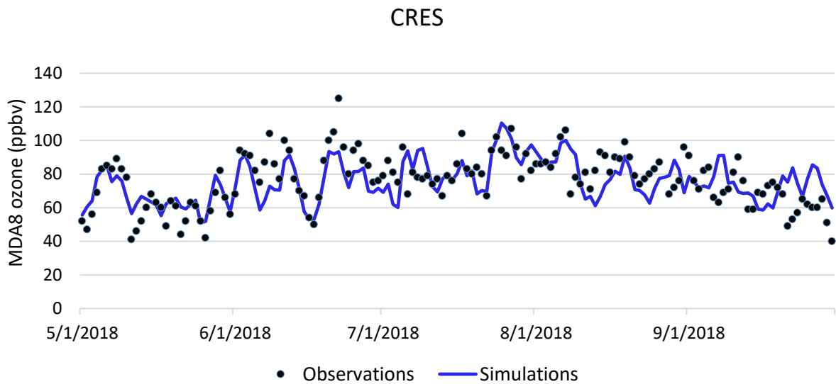
FIGURE III-A-6 2018 MDA8 OZONE MODEL PREDICTION AND MEASUREMENT COMPARISON AT CRESTLINE
