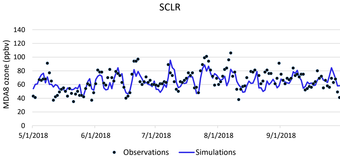
FIGURE III-A-22 2018 MDA8 OZONE MODEL PREDICTION AND MEASUREMENT COMPARISON AT SANTA CLARITA
