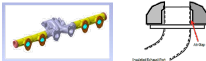
Figure III-6: Insulated Exhaust System
