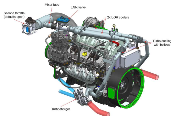
Figure 1: Engine Concept
