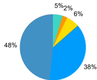
PM10 Emissions: 158 tons/day
