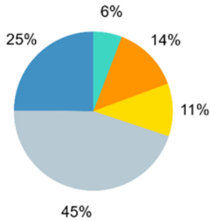
SOx Emissions: 16 tons/day
