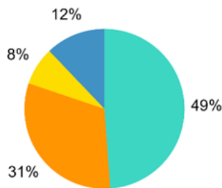
SOx Emissions: 16 tons/day
