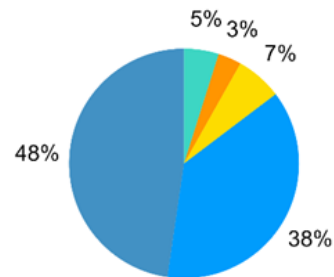
PM10 Emissions: 152 tons/day
