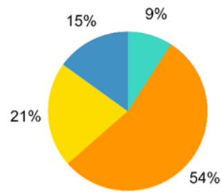
NOx Emissions: 186 tons/day
