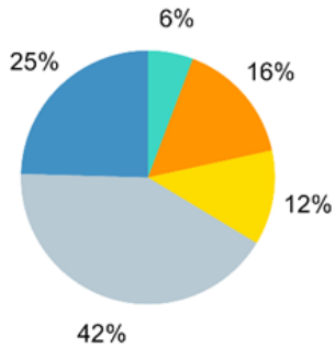
SOx Emissions: 15 tons/day
