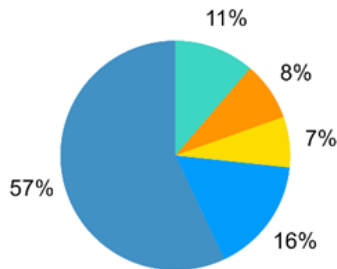
PM2.5 Emissions: 53 tons/day
