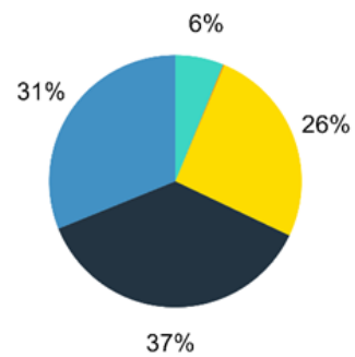
PM10 Emissions: 156 tons/day
