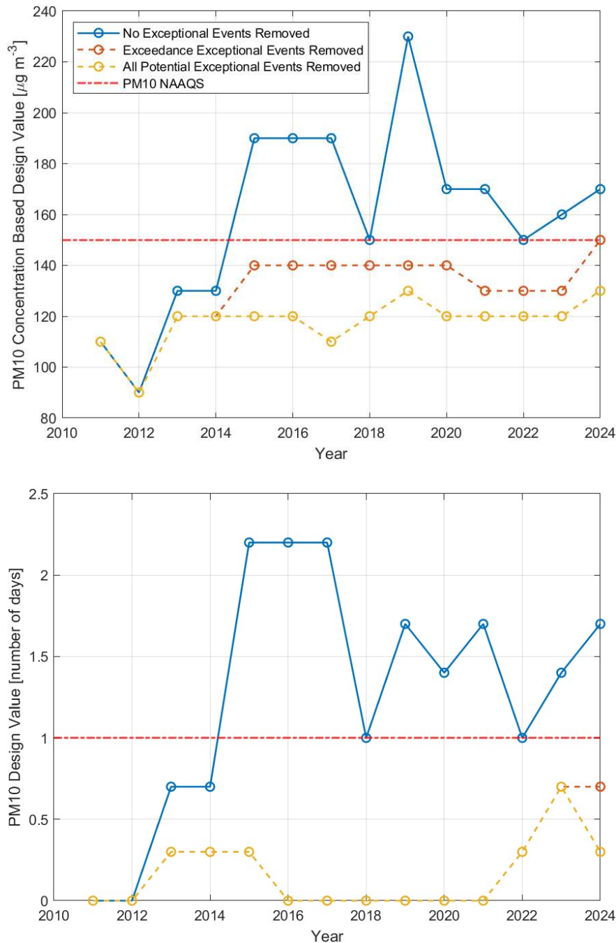
FIGURE 6-1 TREND OF PM10 CONCENTRATION-BASED DESIGN VALUES (TOP) AND DESIGN VALUE (BOTTOM). THE VALUE SHOWN IS THE MAXIMUM OF ALL PM10 MONITORS IN THE SOUTH COAST AIR BASIN. 87
