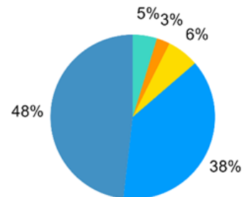
PM10 Emissions: 156 tons/day
