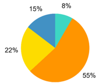
NOx Emissions: 203 tons/day
