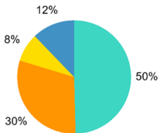
SOx Emissions: 15 tons/day
