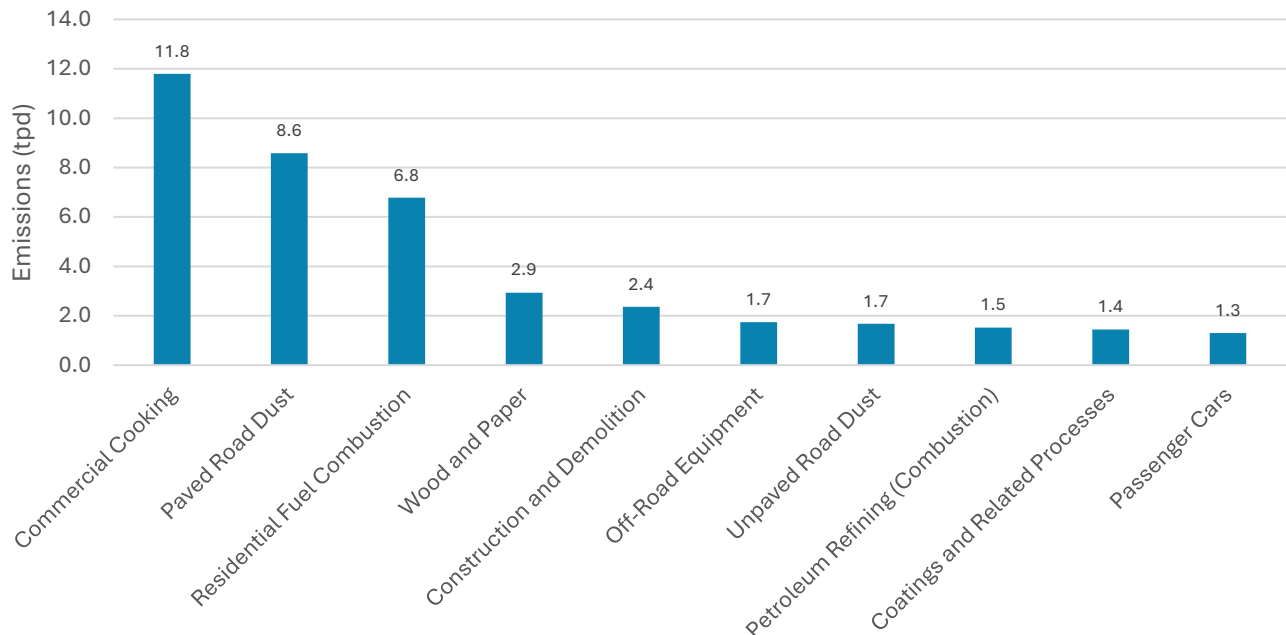
FIGURE III-4 TOP 10 PM 2.5 SOURCES IN 2023
