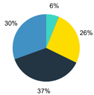
PM10 Emissions: 158 tons/day
