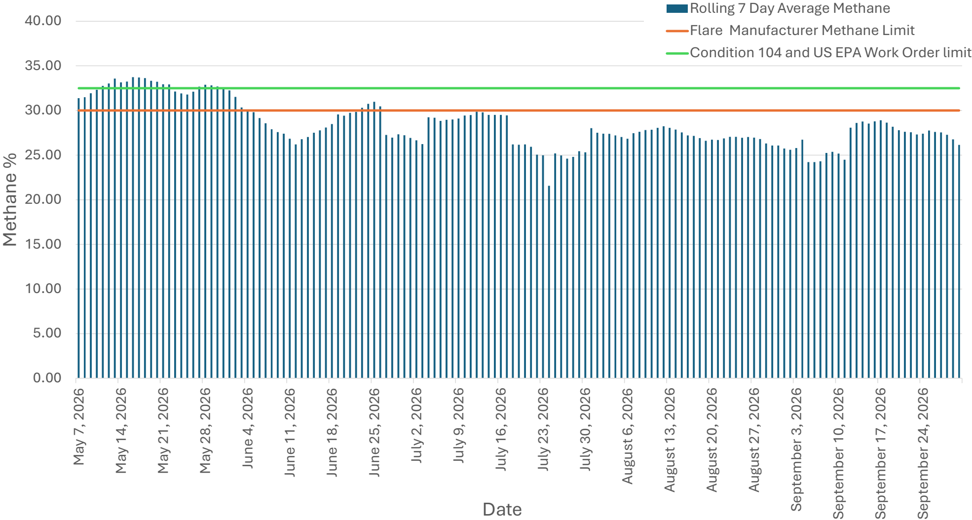
Flare Station Methane Levels (per ASTM Lab Method D1946)
