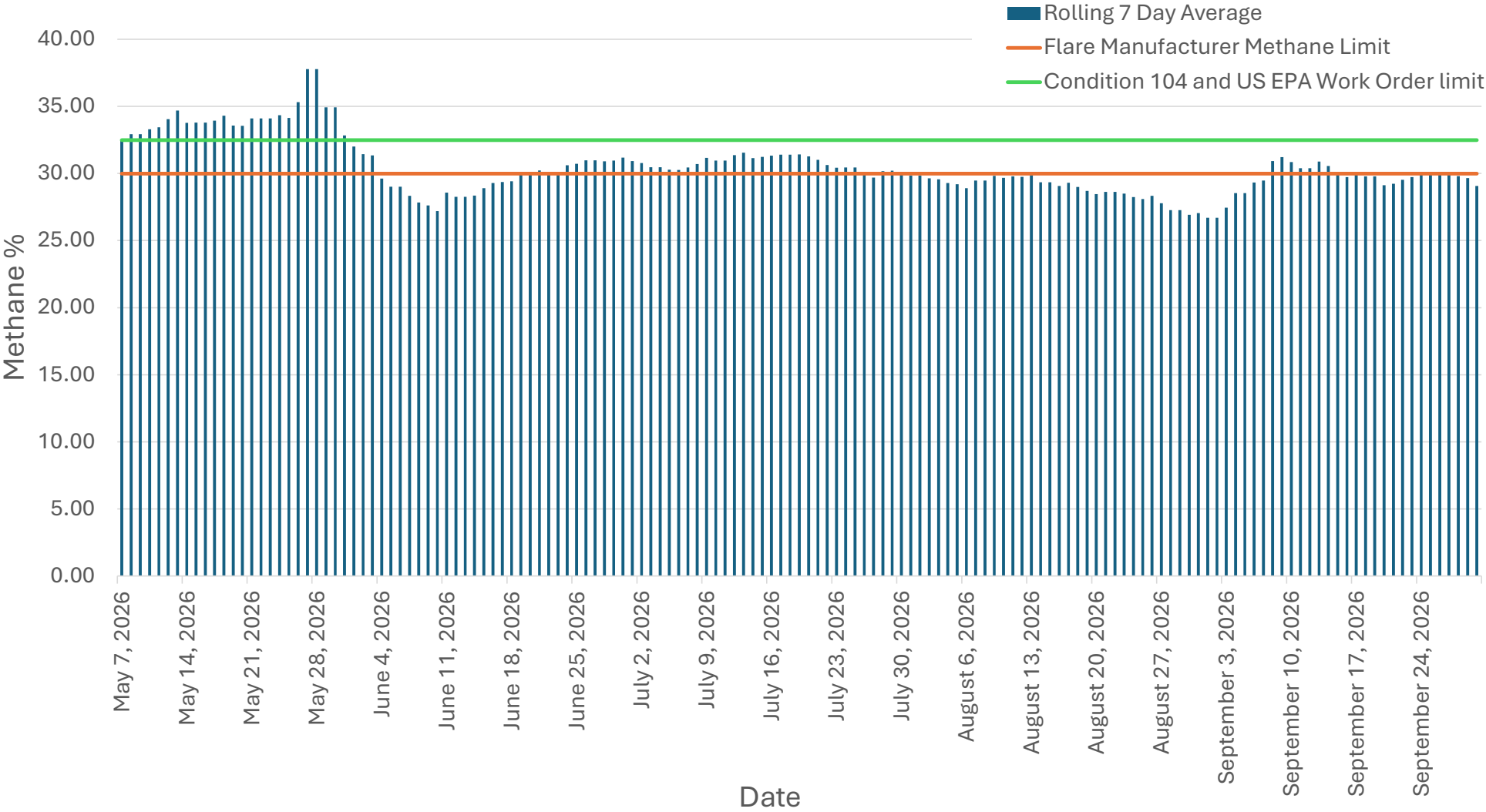
Flare Station Methane Levels (per Handheld Instrument)
