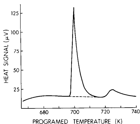
Fig. 3. DSC peak from a calibration experiment (8 mg of zinc was heated at 1 atm with 3 cc min -1 flow of argon).
