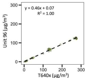
PM 1.0 GGSensors – TAM vs T640x (5-minute mean, µg/m 3 )
