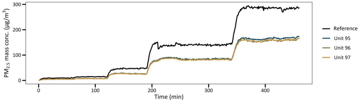
Timeseries of PM 2.5 Concentration Ramp
