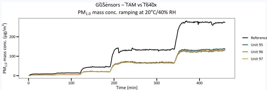
PM 1.0 GGSensors – TAM vs T640x (5-minute mean, µg/m 3 )
