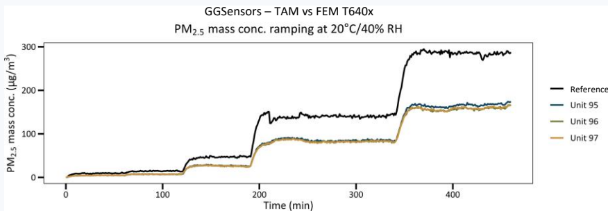
PM 2.5 GGSensors – TAM vs FEM T640x (5-minute mean, \mu\text{g}/\text{m}^3 )
