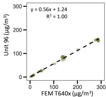
PM 2.5 GGSensors – TAM vs FEM T640x (5-minute mean, \mu\text{g}/\text{m}^3 )
