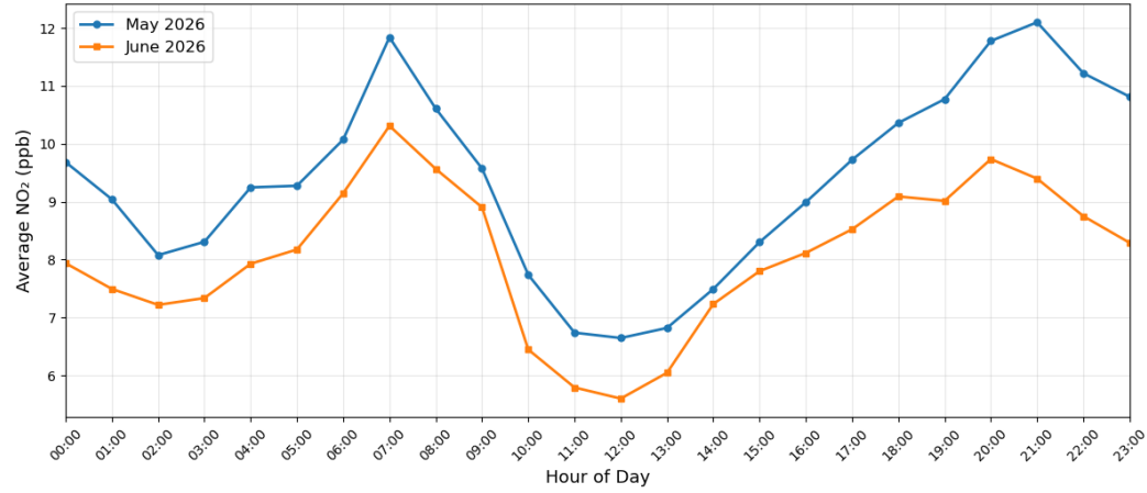
Highlander at North Campus Apartment Monitor Average Hourly NO 2 Concentration May & June 2026
