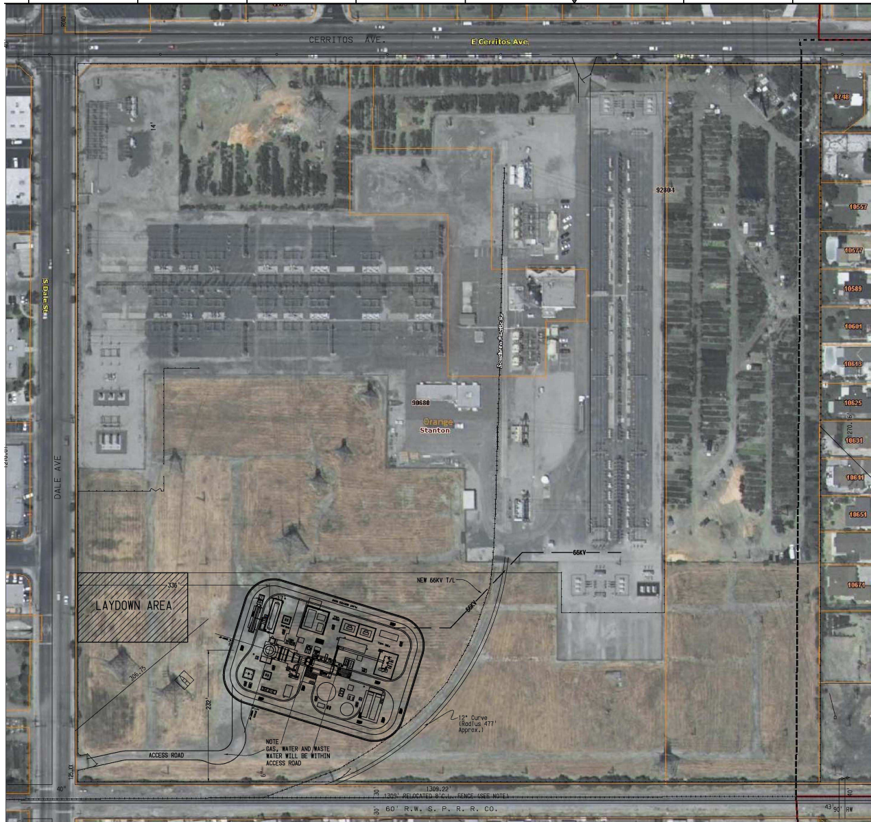
Figure 2 Aerial Photograph of the Facility with Plot Plan [Revised from Draft MND to reflect change in site configuration]
