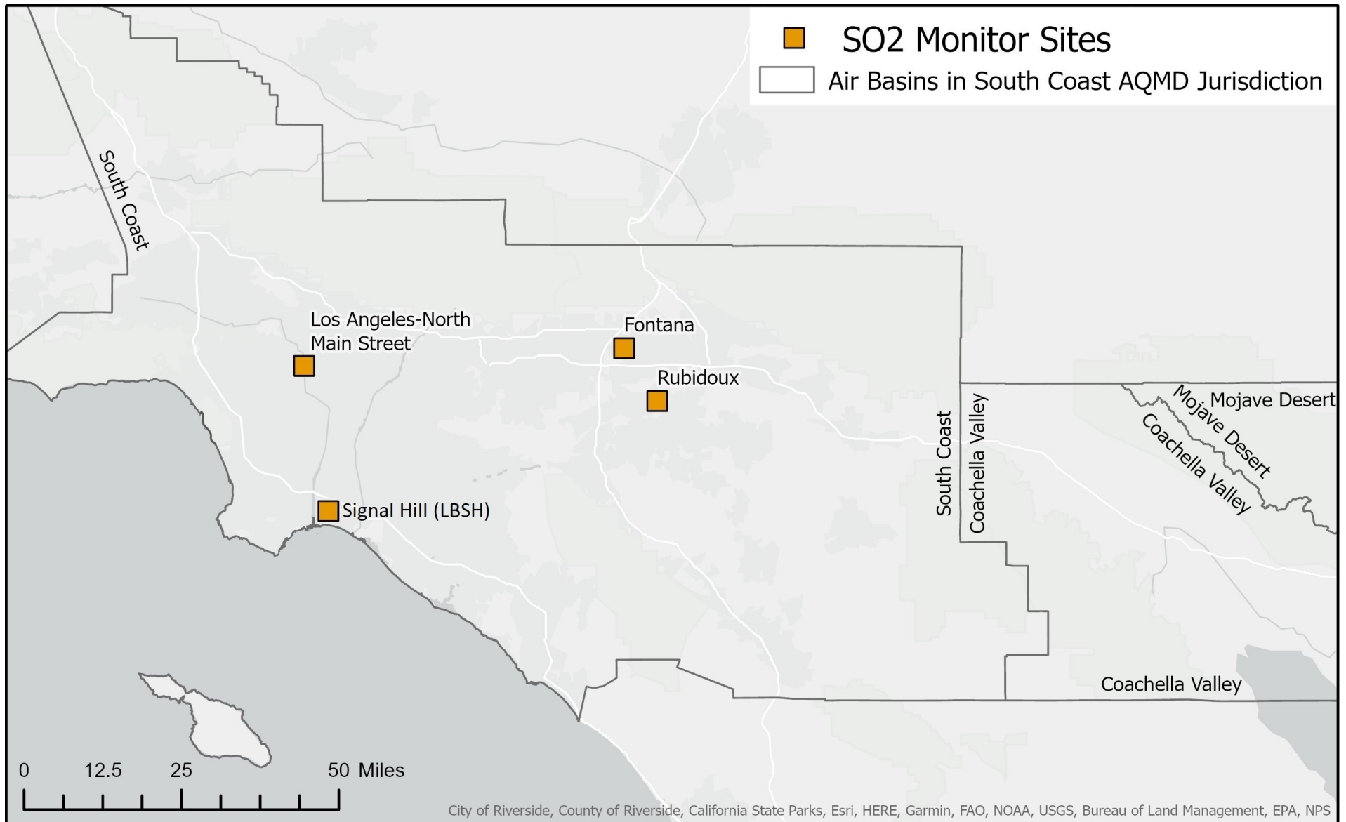
Figure 5 South Coast AQMD Sulfur Dioxide Monitoring Locations
