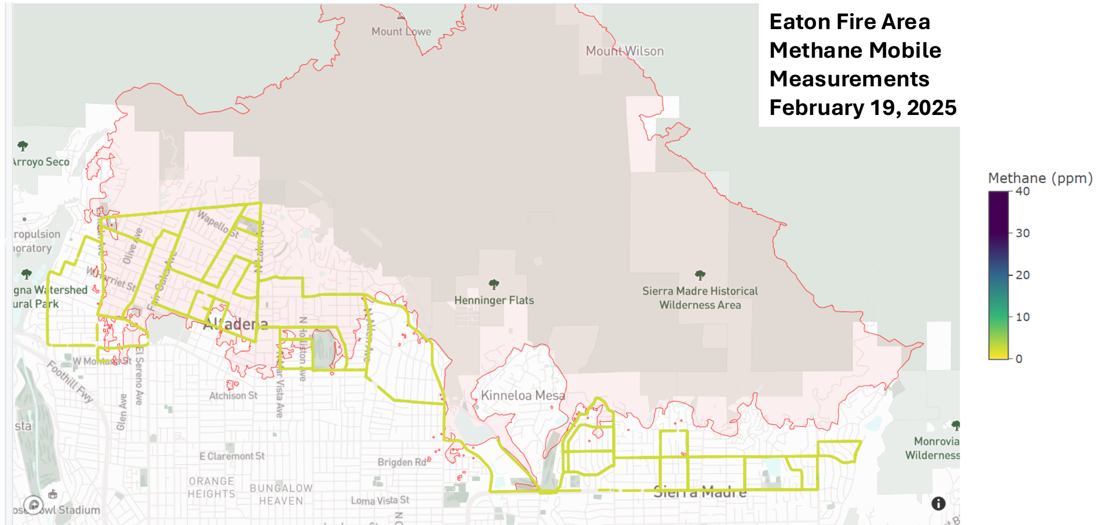
Figure 9. Map shows the concentrations of Methane measured on February 19, 2025.
