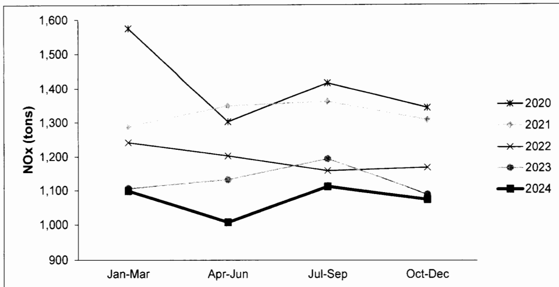
Figure 7-2 Quarterly NOx Emissions from Calendar Years 2020 through 2024
