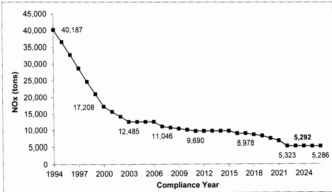
Figure 2-1 NOx RTC Supply
