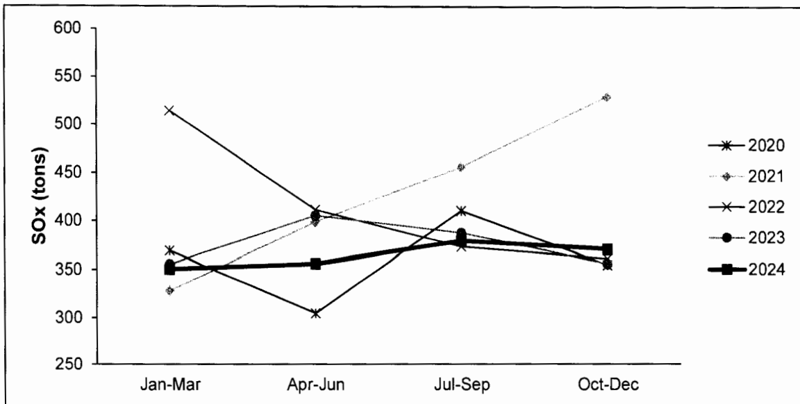
Figure 7-4 Quarterly SOx Emissions from Calendar Years 2020 through 2024
