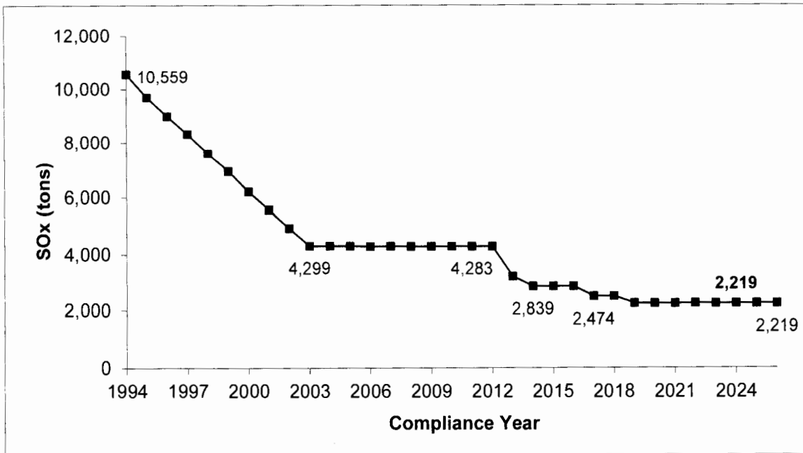
Figure 2-2 SOx RTC Supply
