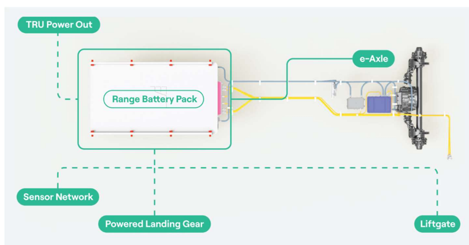
Figure 8: Range Energy Trailer Technology Overview
