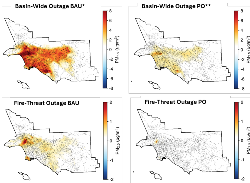
Difference in January PM 2.5 Concentrations Between the 2045 Scenarios and the Baseline Scenario
