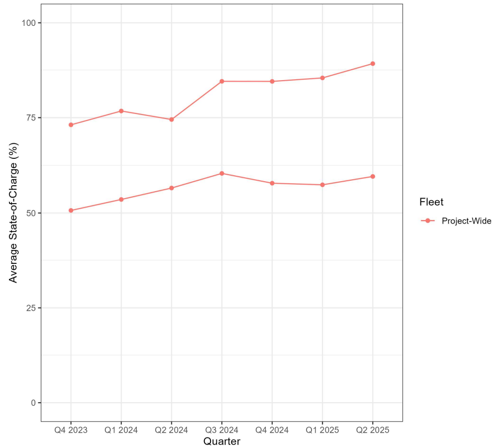
State-of-Charge Ranges Full Project Period Average Maximum and Minimum Daily SOC
